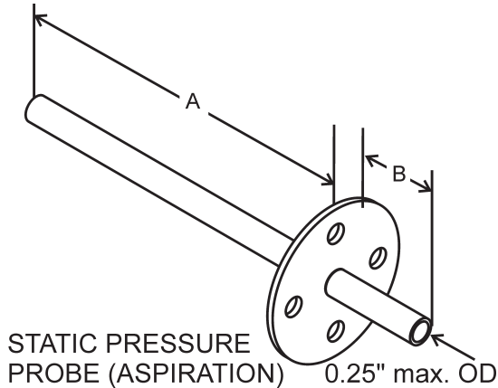
Static Pressure (Aspiration) Probes
