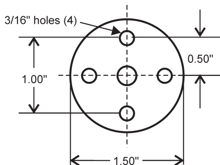
MOUNTING FLANGE
